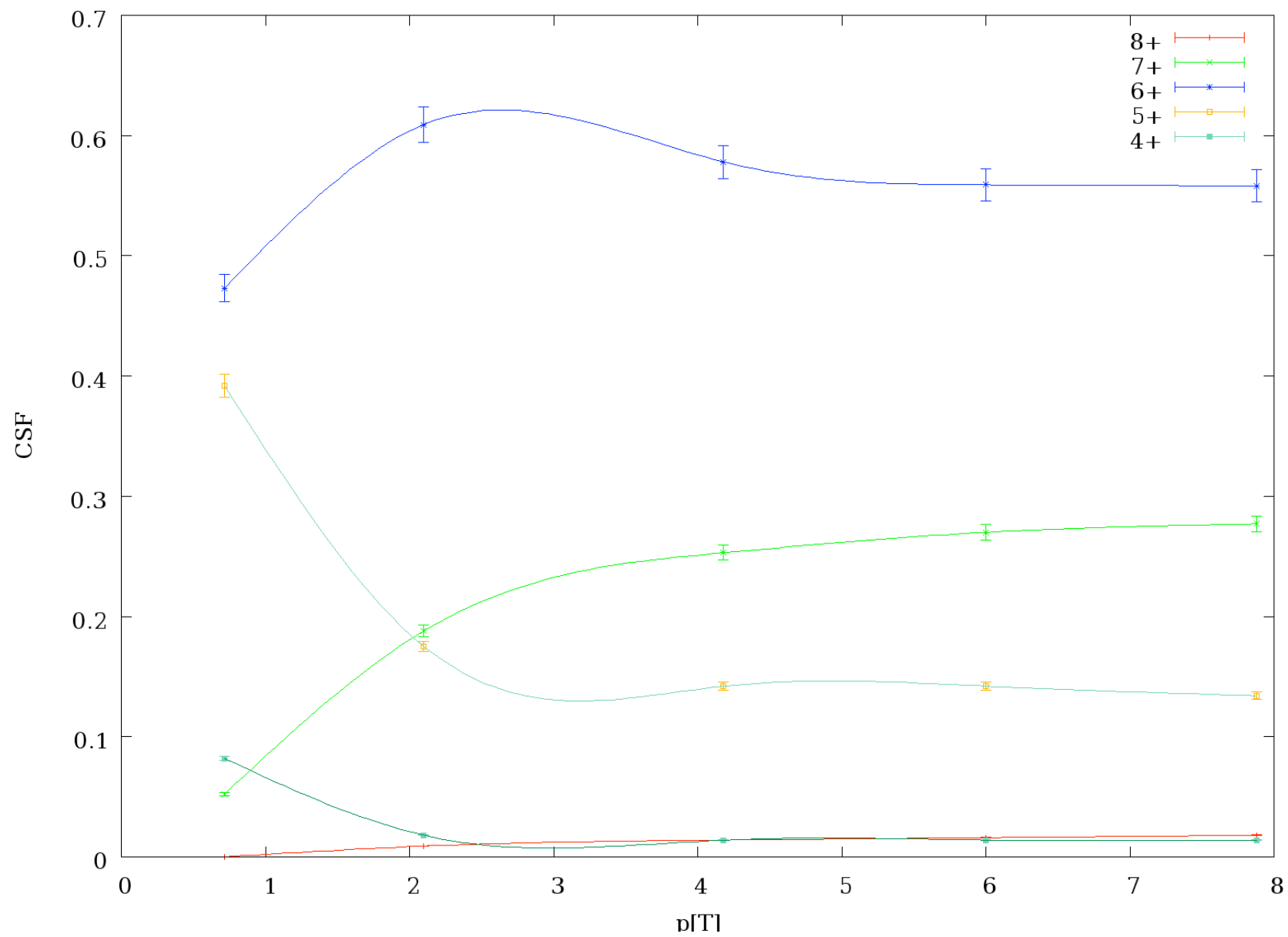
CSD of ^{16}\text{O} (4+) in He at 1.0 MeV/u
