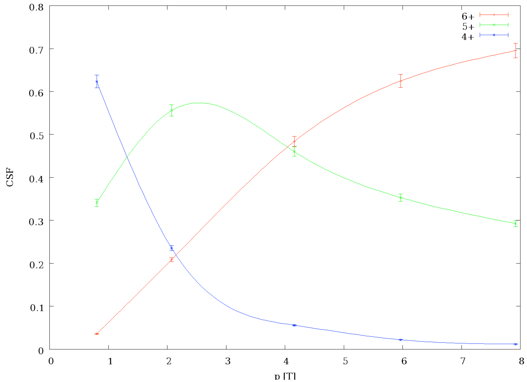
CSD of ^{12}\text{C} ( 3+ ) in He at 1.75 MeV/u
