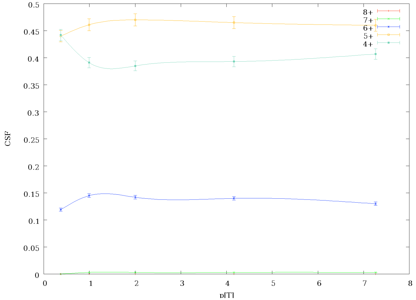
CSD of ^{16}\text{O} ( 4+ ) in He at 0.5 MeV/u
