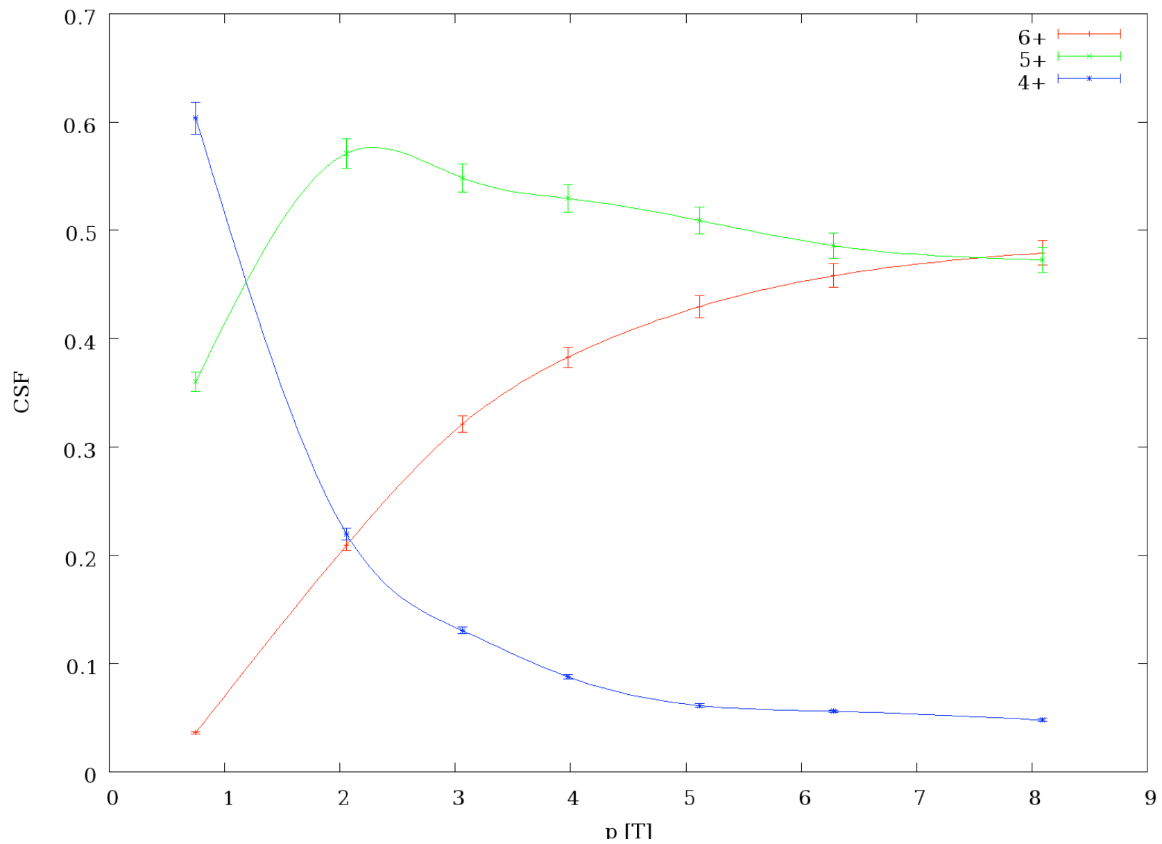
CSD of ^{12}\text{C} (3+) in He at 1.2 MeV/u
