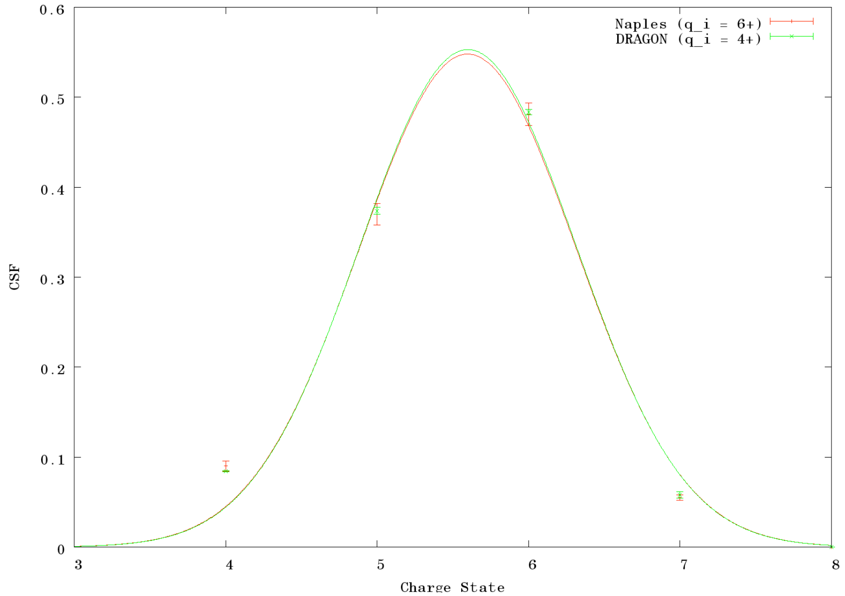
Equilibrium CSD of ^{16}\text{O} in He at 0.75 MeV/u Comparison with Data from Naples
