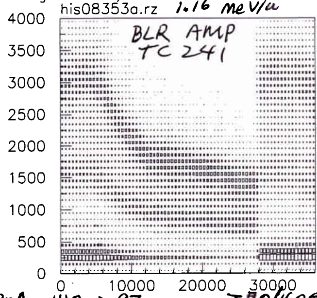
H-Run-time x Elastic-energy his08353a.rz
